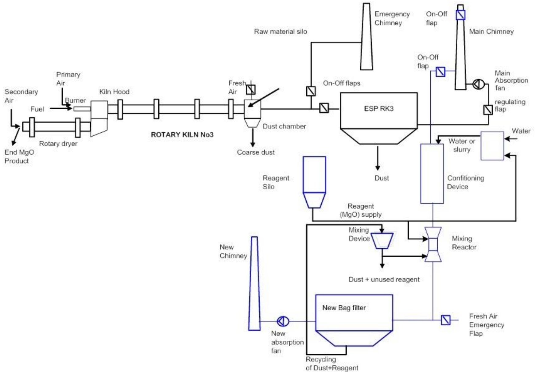
Figure 1. Demonstration plant process flow sheet (in blue) being fed the flue gases from rotary kiln No.2
